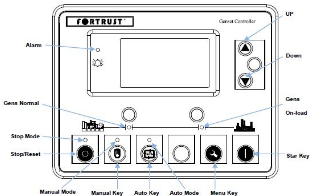
GEC7010C panel indicators
